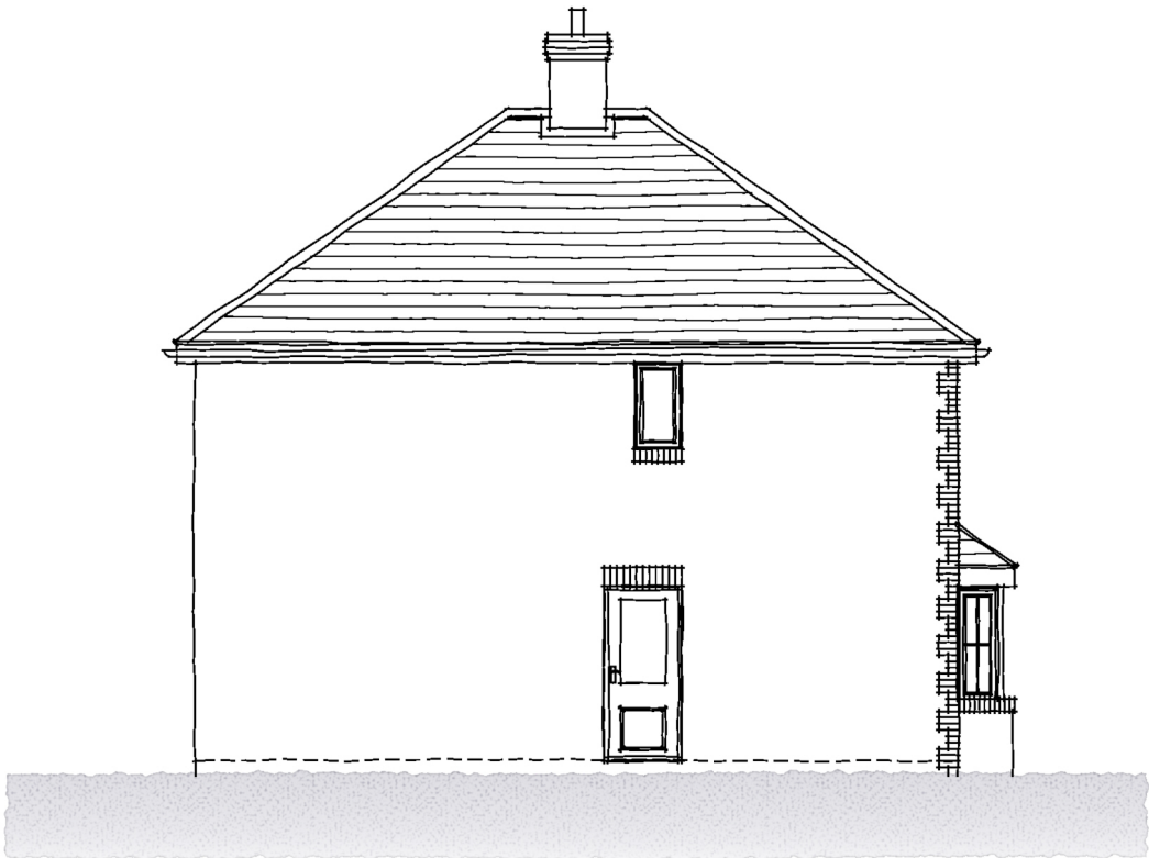
REAR ELEVATION
