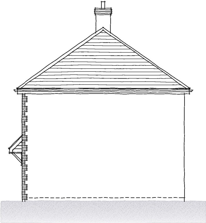
SIDE ELEVATION
