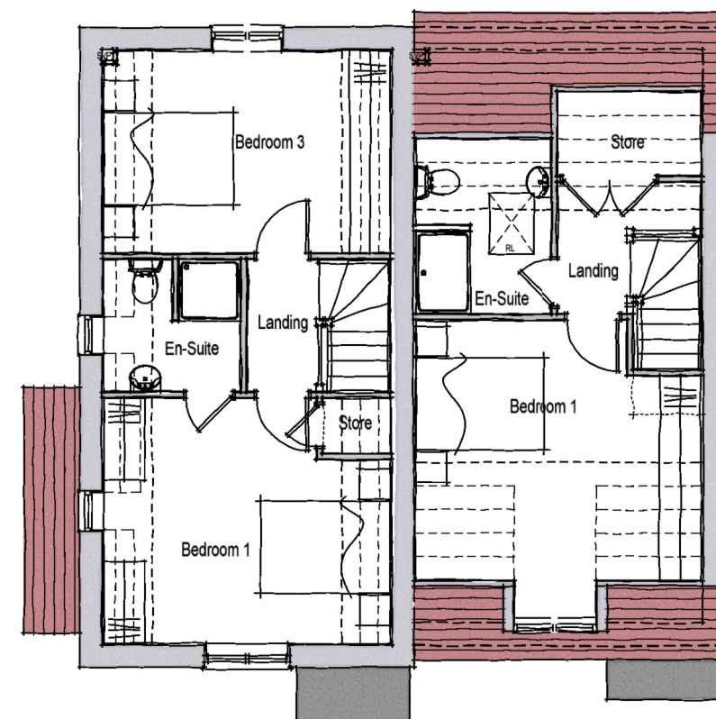
SECOND FLOOR PLAN TYPE P2 TYPE P
