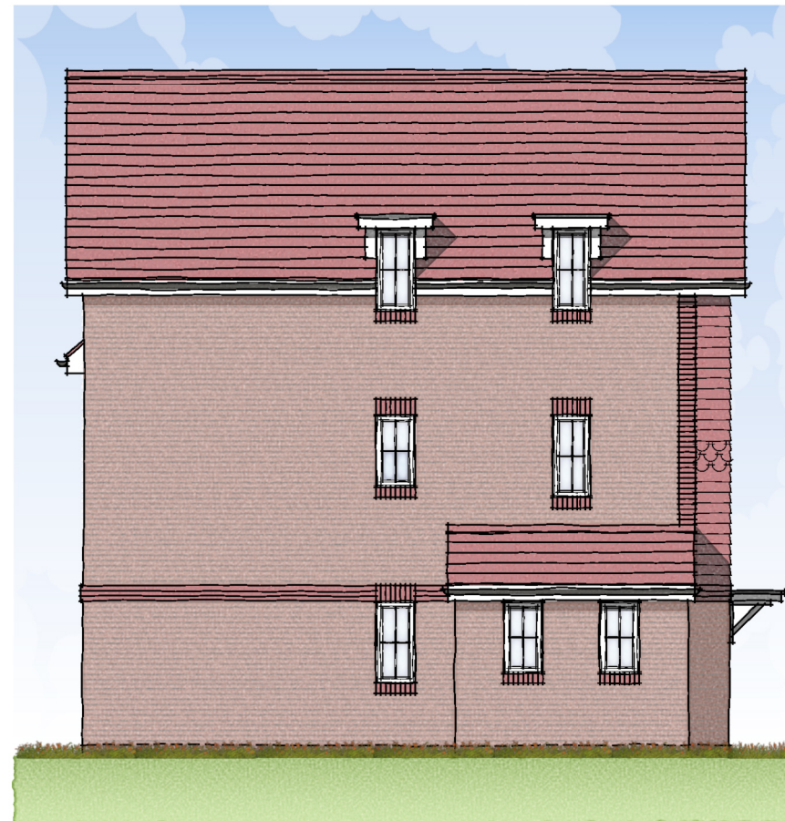
SIDE ELEVATION TYPE P2
