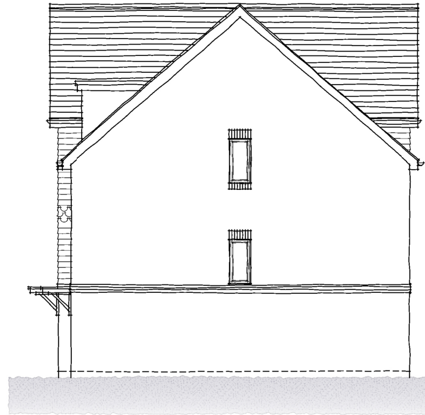
SIDE ELEVATION TYPE P
