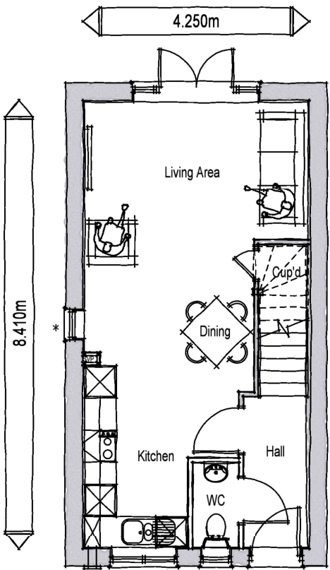
GROUND FLOOR PLAN *WINDOW FOR PLOT 342 ON
