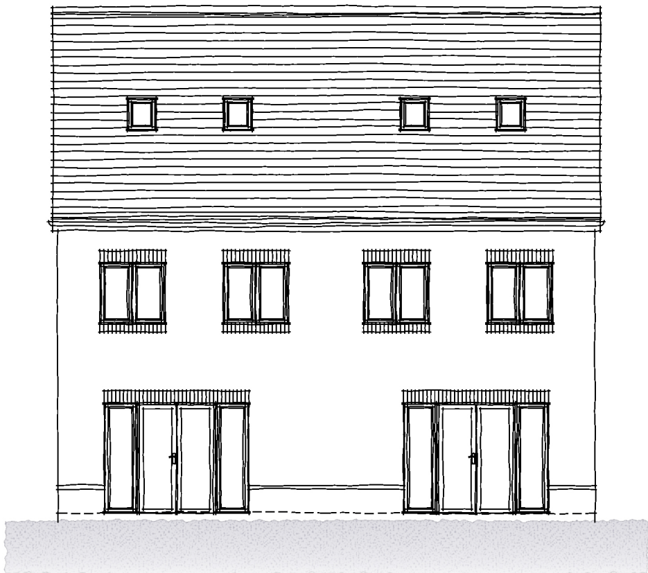
REAR ELEVATION
