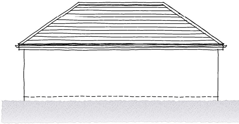
REAR ELEVATION
