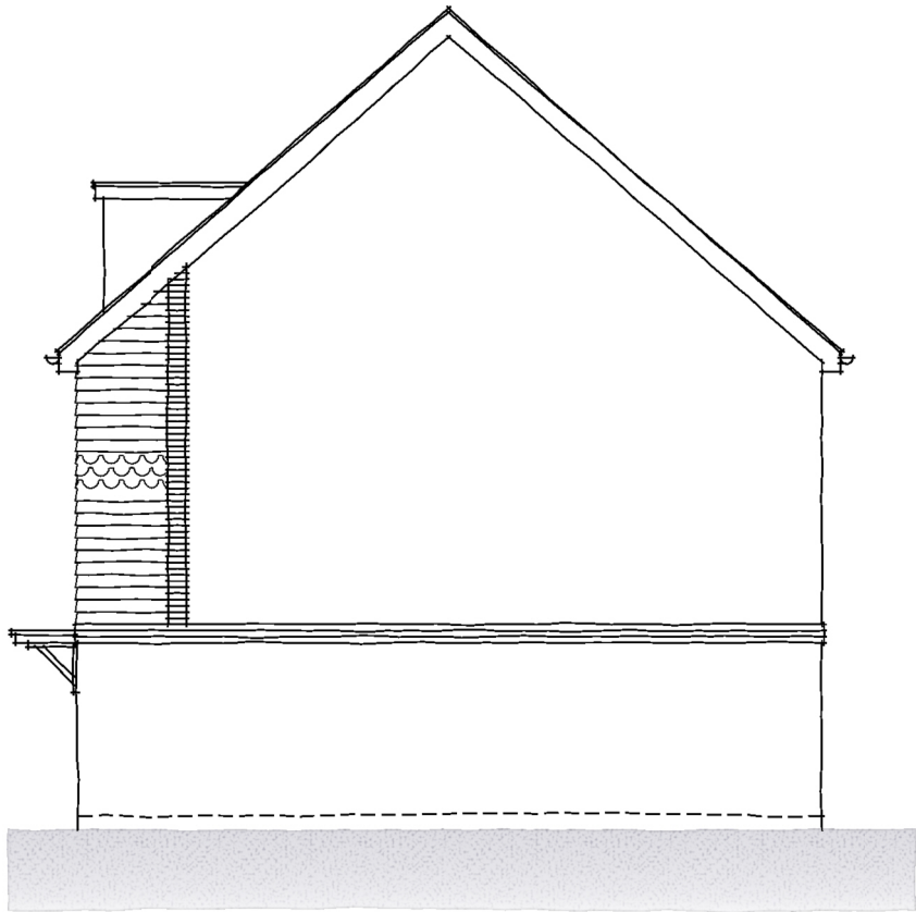
SIDE ELEVATION
