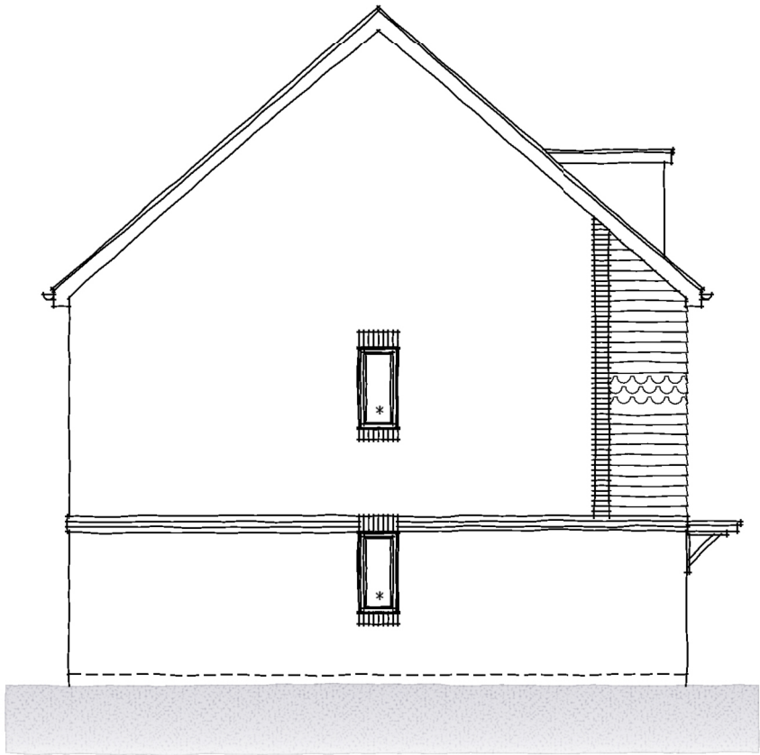
SIDE ELEVATION *REMOVE WINDOW FOR PLOT 123
