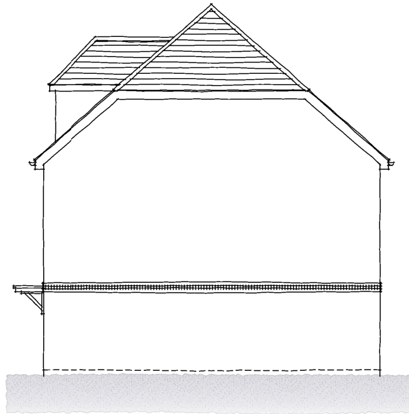
SIDE ELEVATION
