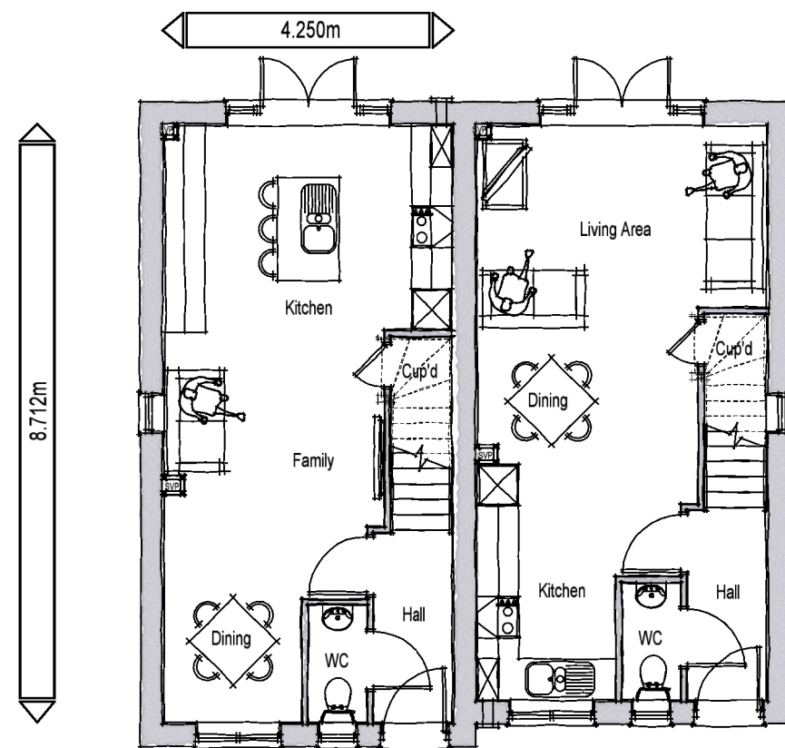
GROUND FLOOR PLAN TYPE P3 TYPE P
