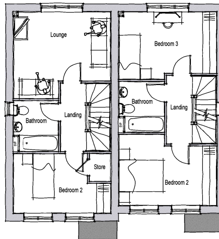
FIRST FLOOR PLAN TYPE P3 TYPE P
