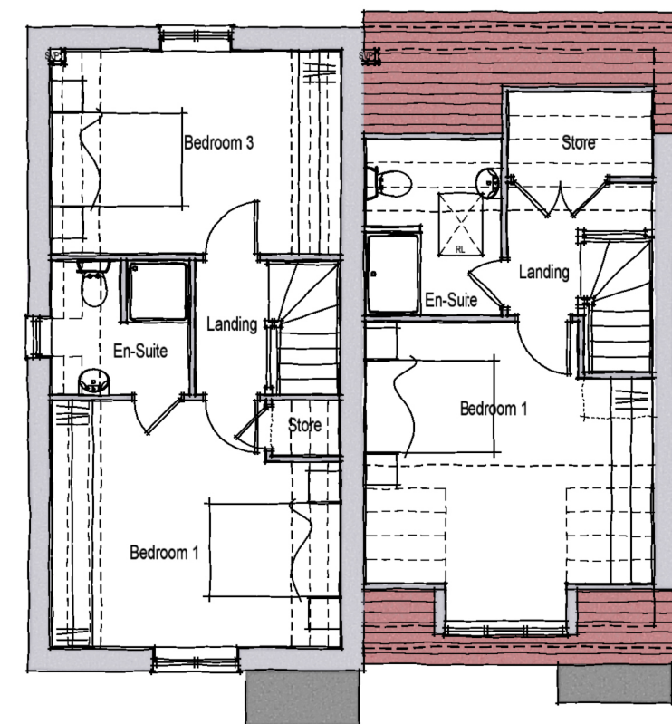
SECOND FLOOR PLAN TYPE P3 TYPE P
