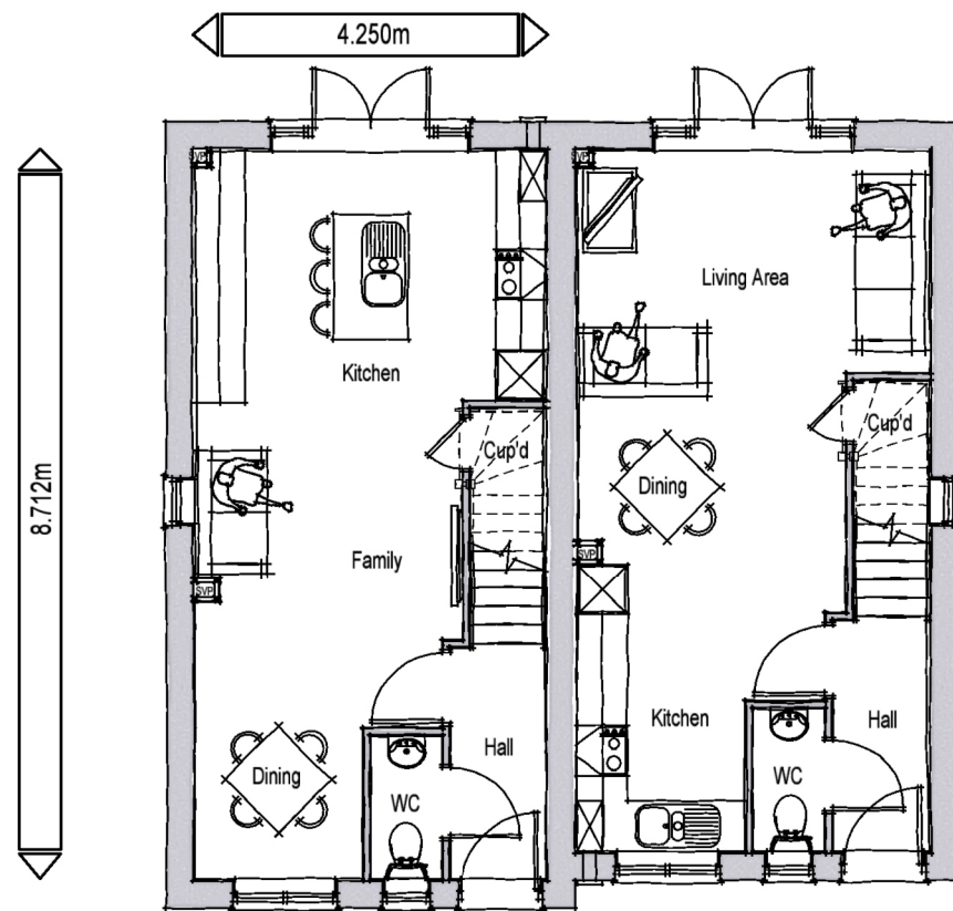
GROUND FLOOR PLAN TYPE P3 TYPE P
