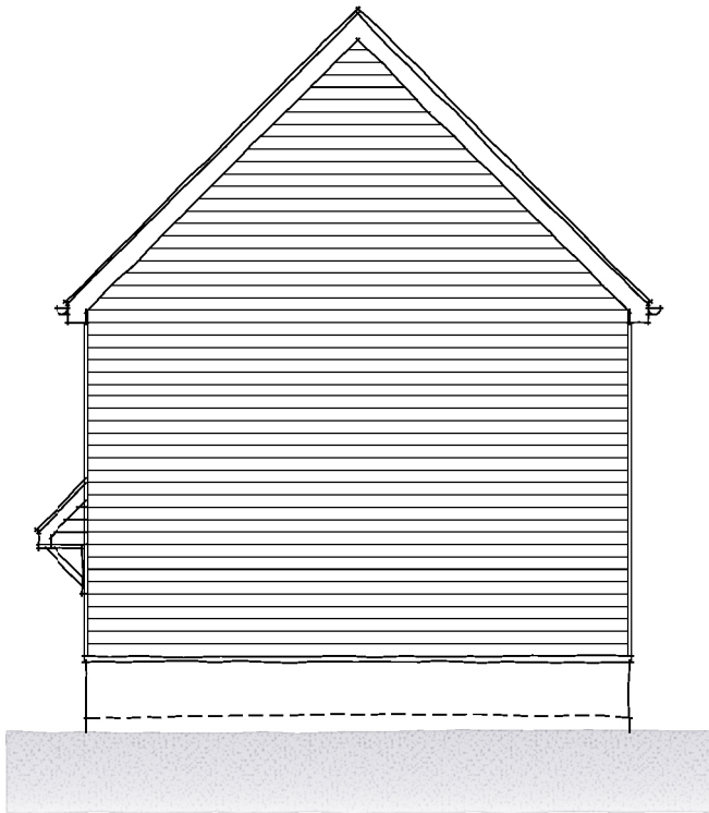
SIDE ELEVATION
