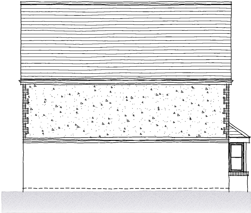
REAR ELEVATION
