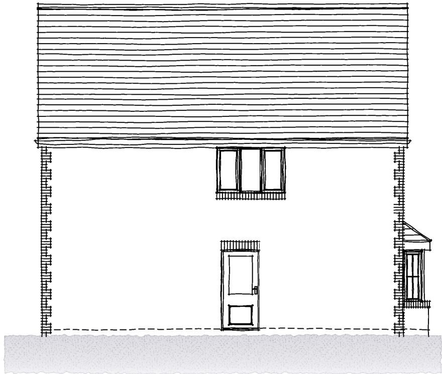
REAR ELEVATION
