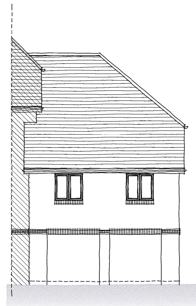
REAR ELEVATION
