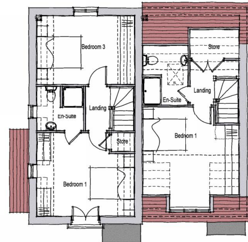
SECOND FLOOR PLAN TYPE P2 TYPE P
