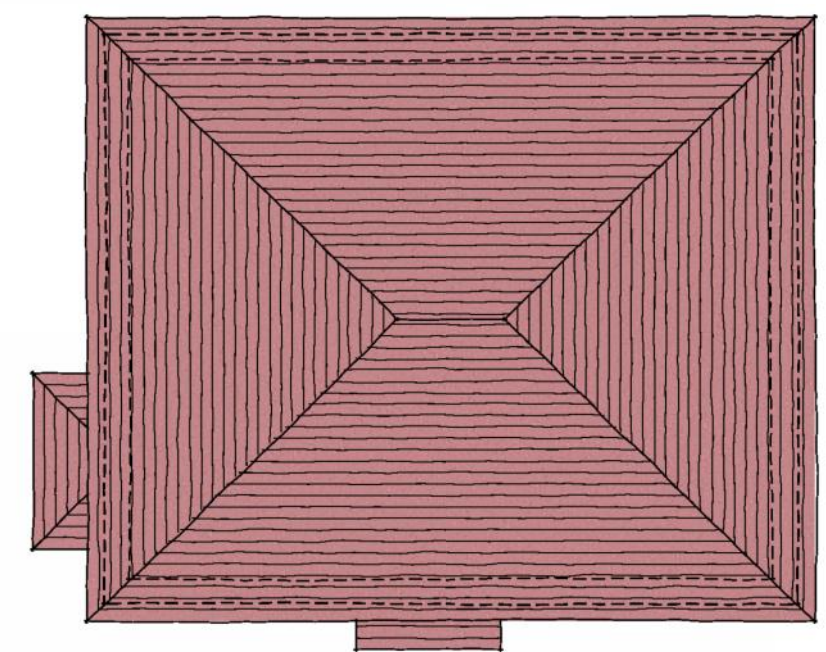
ROOF PLAN
