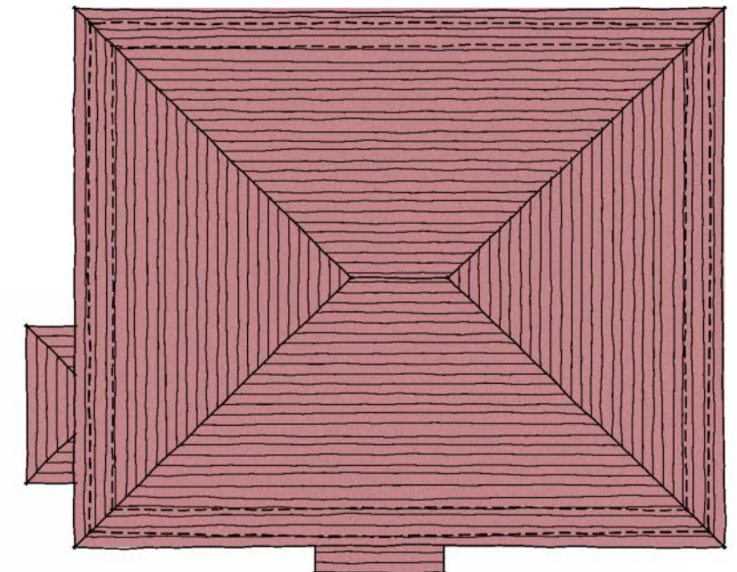
ROOF PLAN
