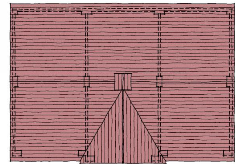
ROOF PLAN
