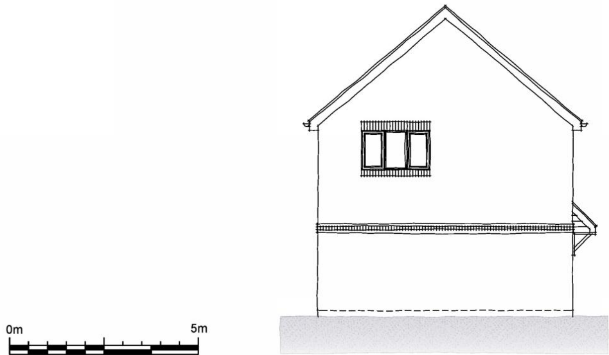
SIDE ELEVATION
