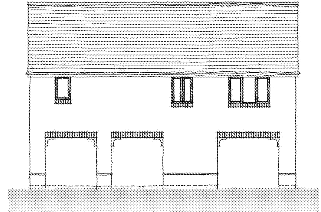
REAR ELEVATION
