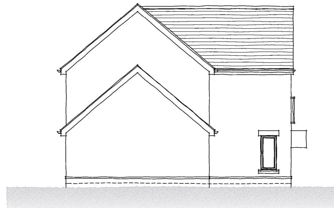
SIDE ELEVATION
