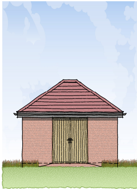
FRONT ELEVATION
