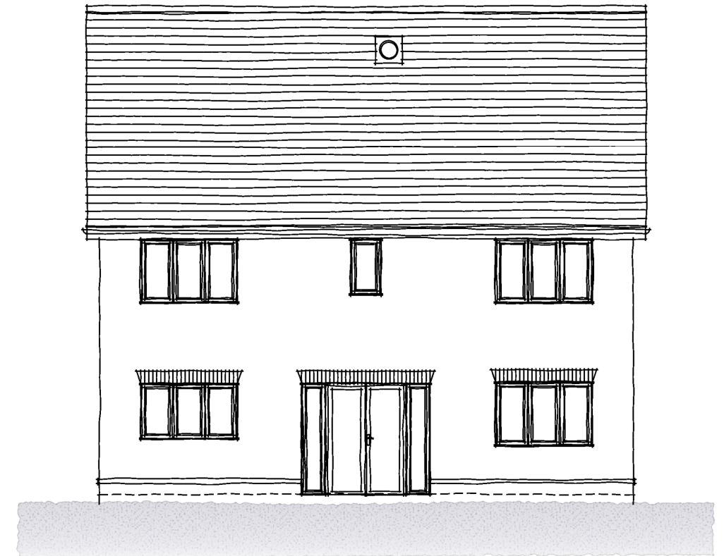
REAR ELEVATION
