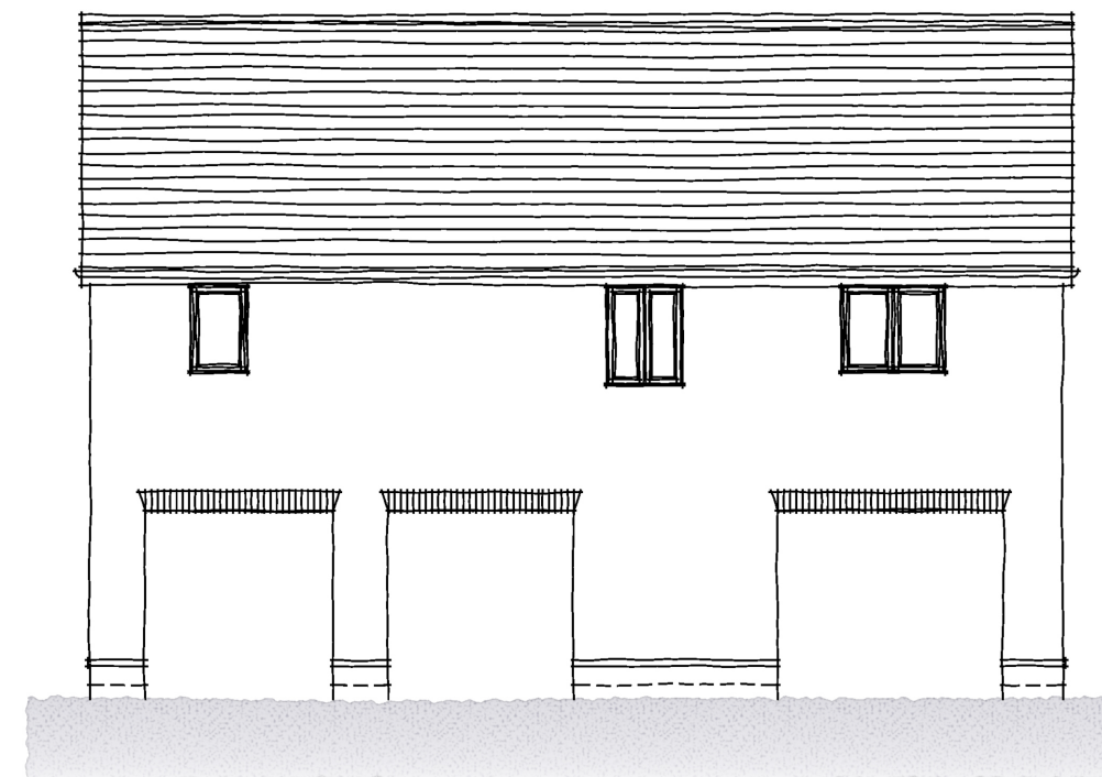
REAR ELEVATION
