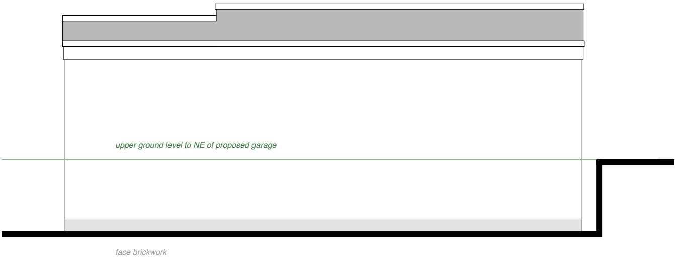
Proposed Rear Elevation at 1:50 scale NORTH EAST
