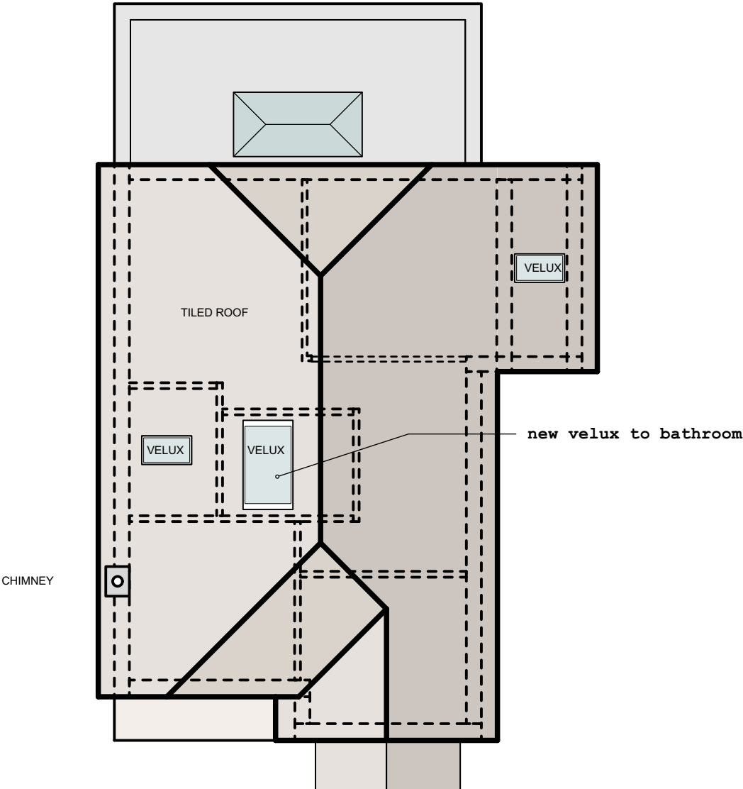
roof plan:
