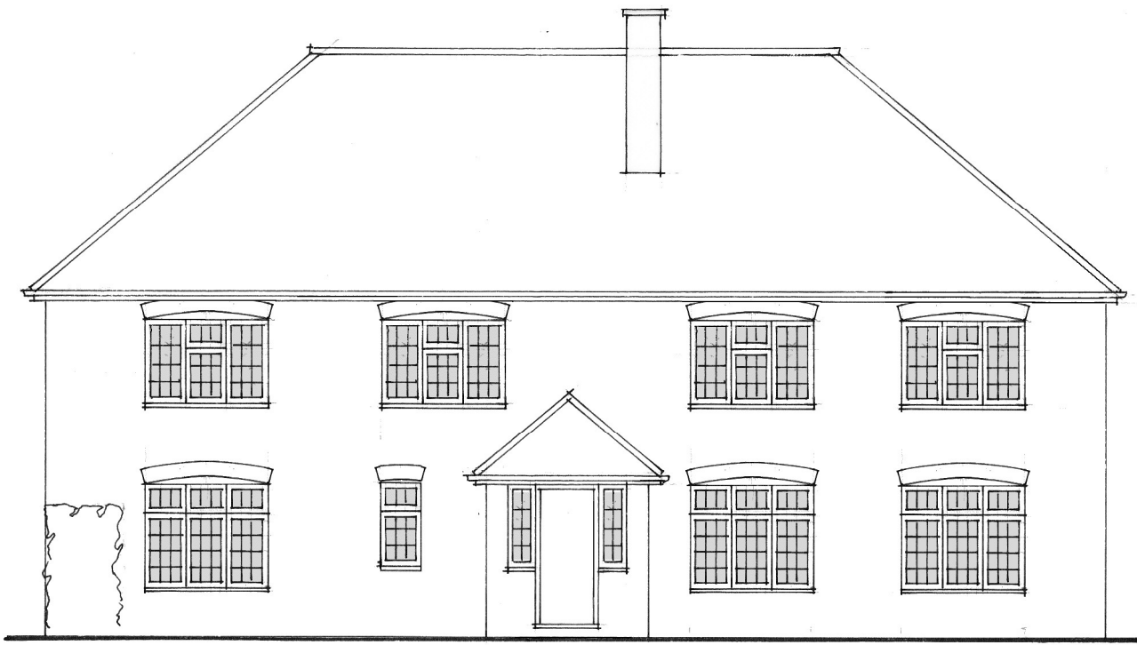
WEST ELEVATION
