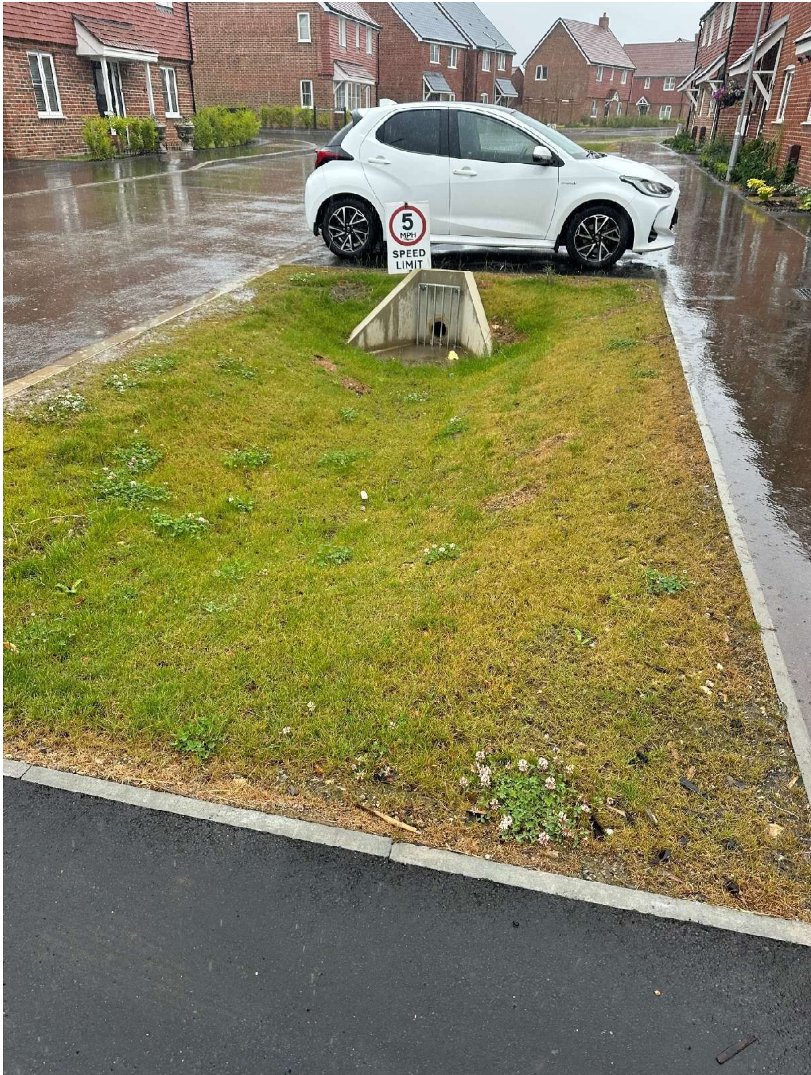
Swale R-HW2G - 9 July 2024 - complete and functioning
