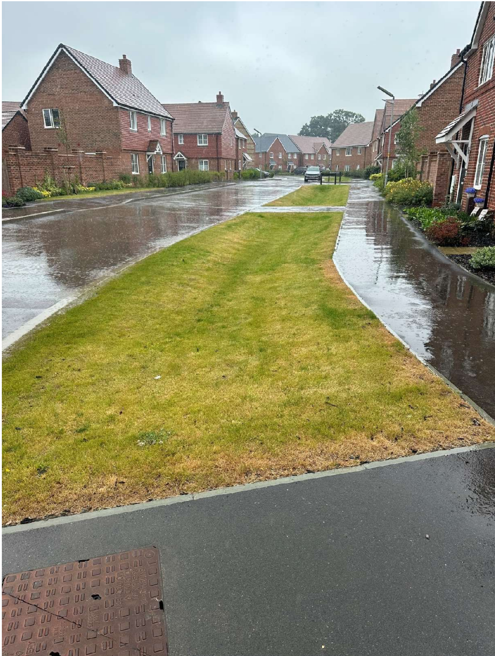
Swale O-N - 9 July 2024 - complete and functioning
