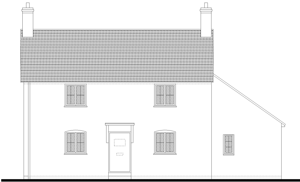
Existing Front Elevation at 1:100 scale SOUTH WEST
