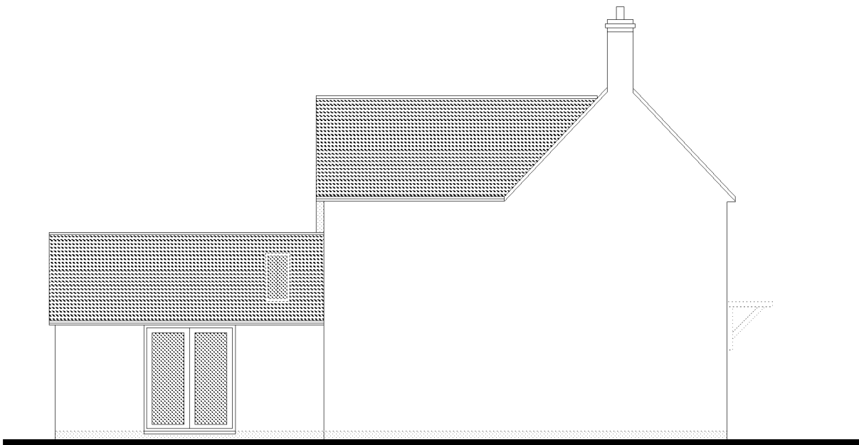
Existing Side Elevation at 1:100 scale NORTH EAST
