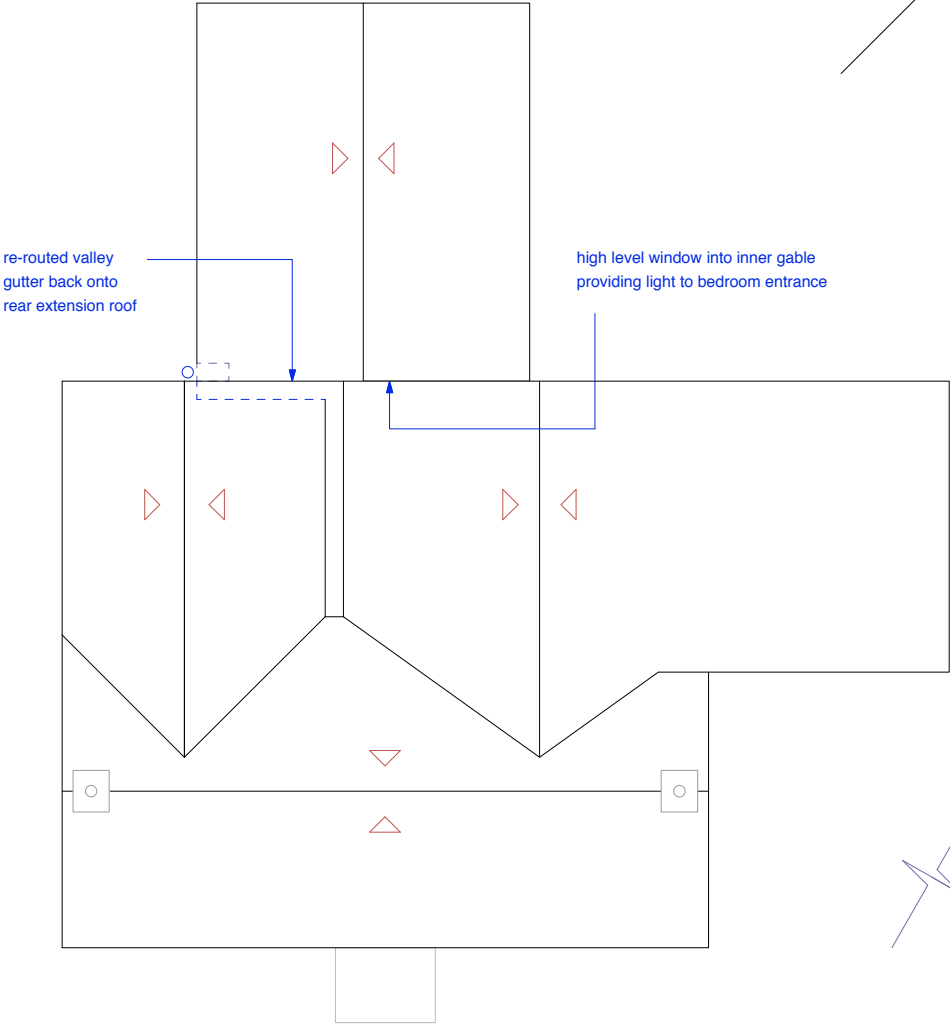
Proposed Roof Plan at 1:100 scale
