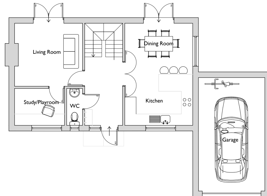
Ground Floor Plan 1:100 @ A3
