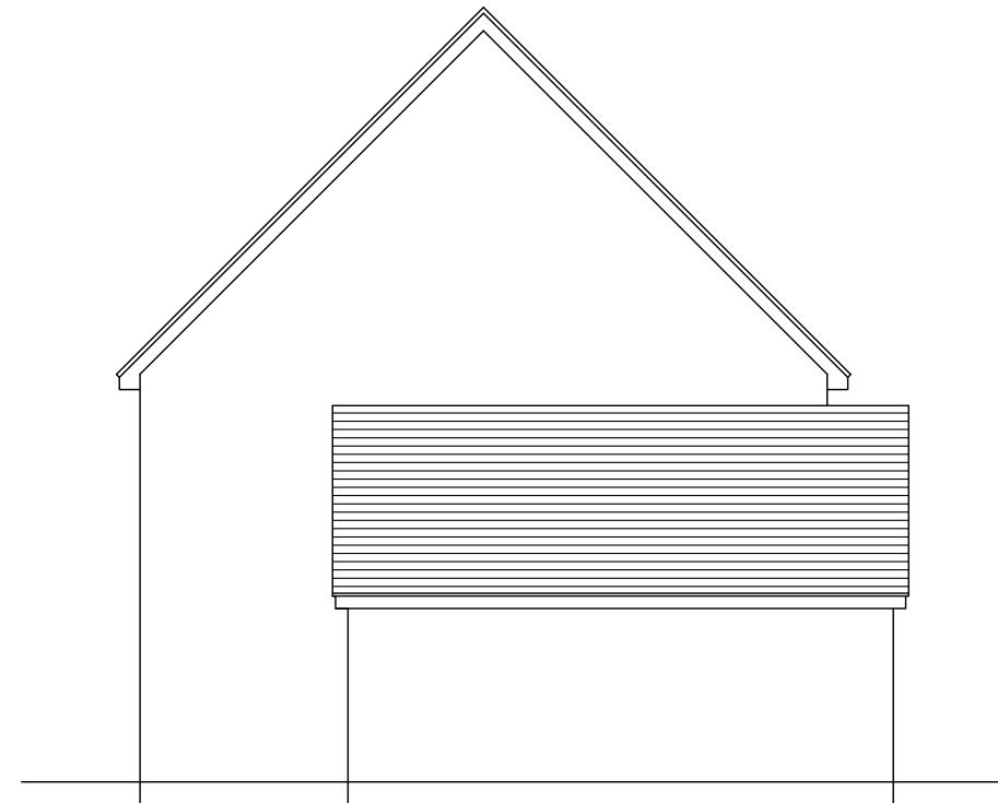
East Elevation 1:100 @ A3
