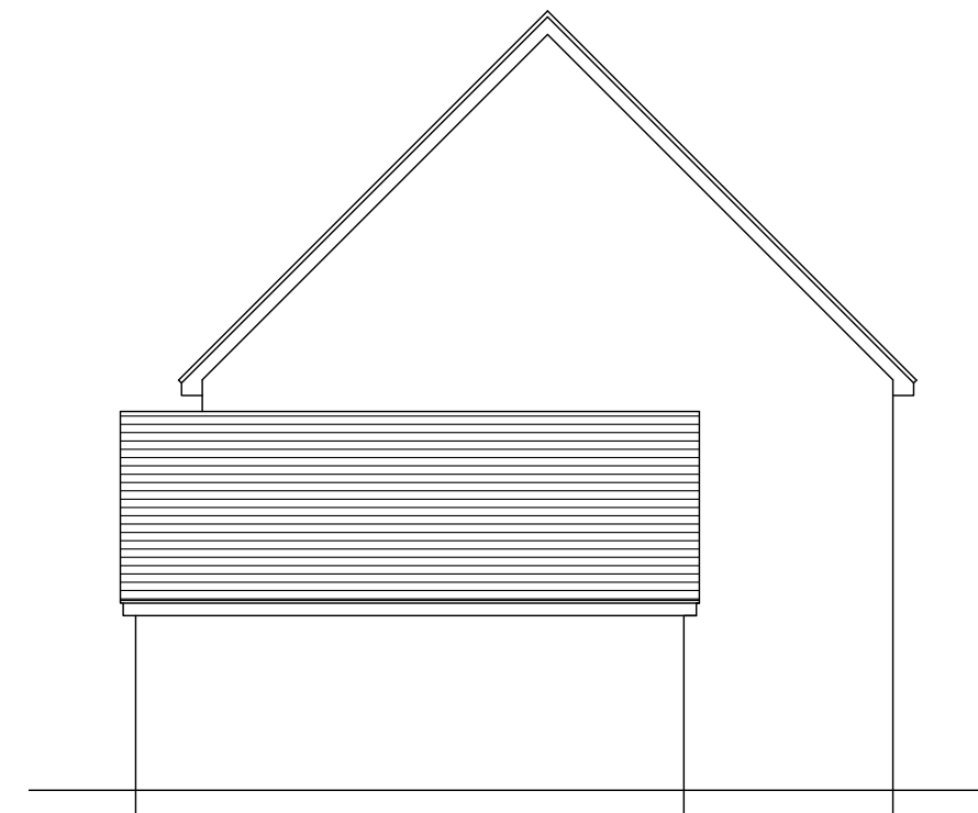
West Elevation 1:100 @ A3
