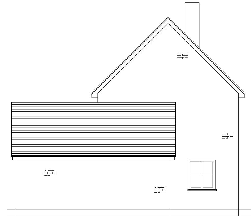
East Elevation 1:100 @ A3
