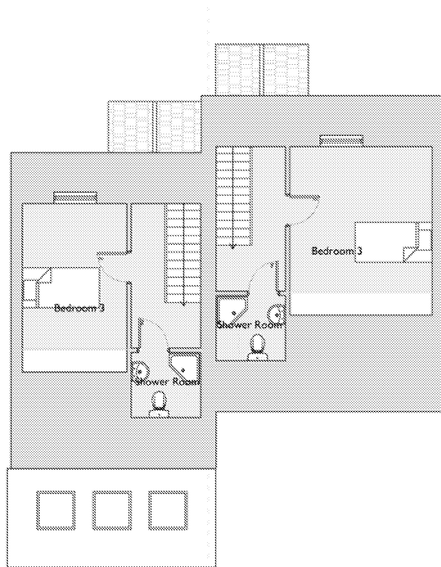
Second Floor Plan 1:100 @ A3
