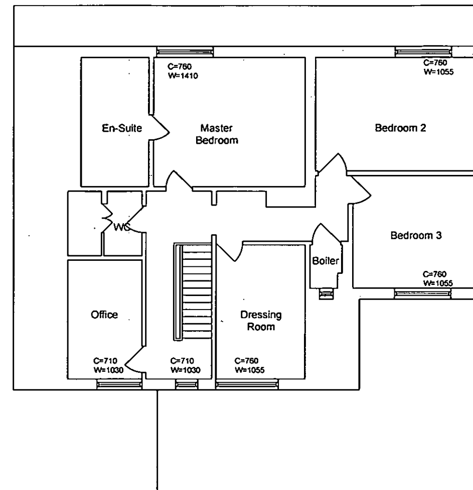
First Floor Plan 1:100 @ A3
