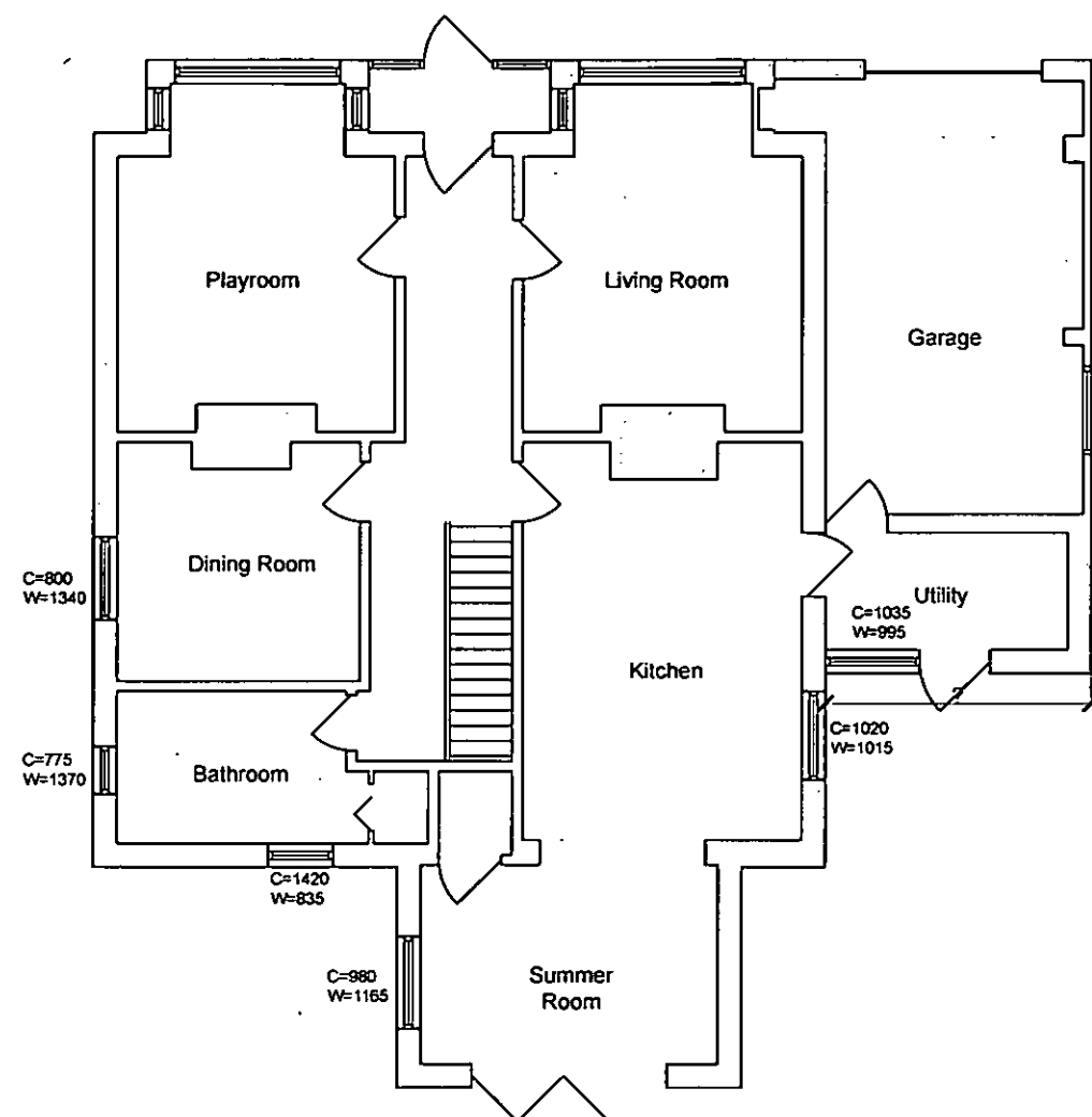
Existing Ground Floor Plan 1:100 @ A3
