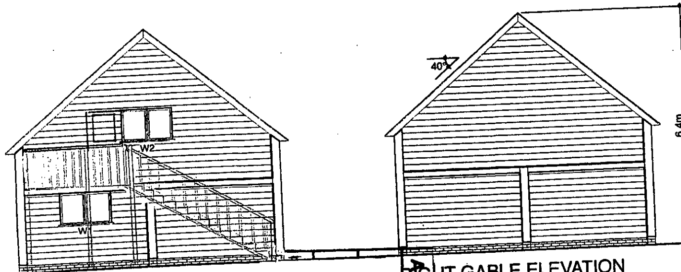
LEFT GABLE ELEVATION
