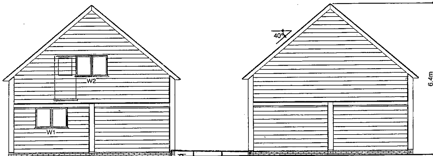
RIGHT GABLE ELEVATION
