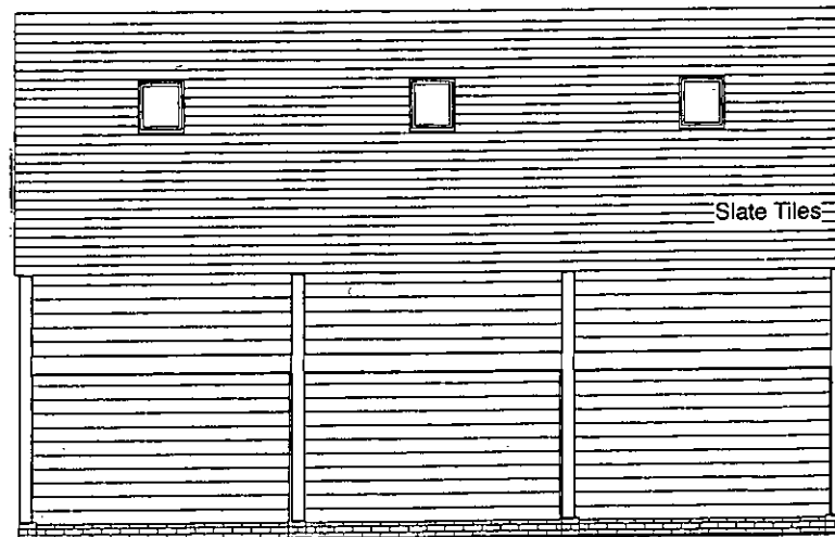
REAR ELEVATION
