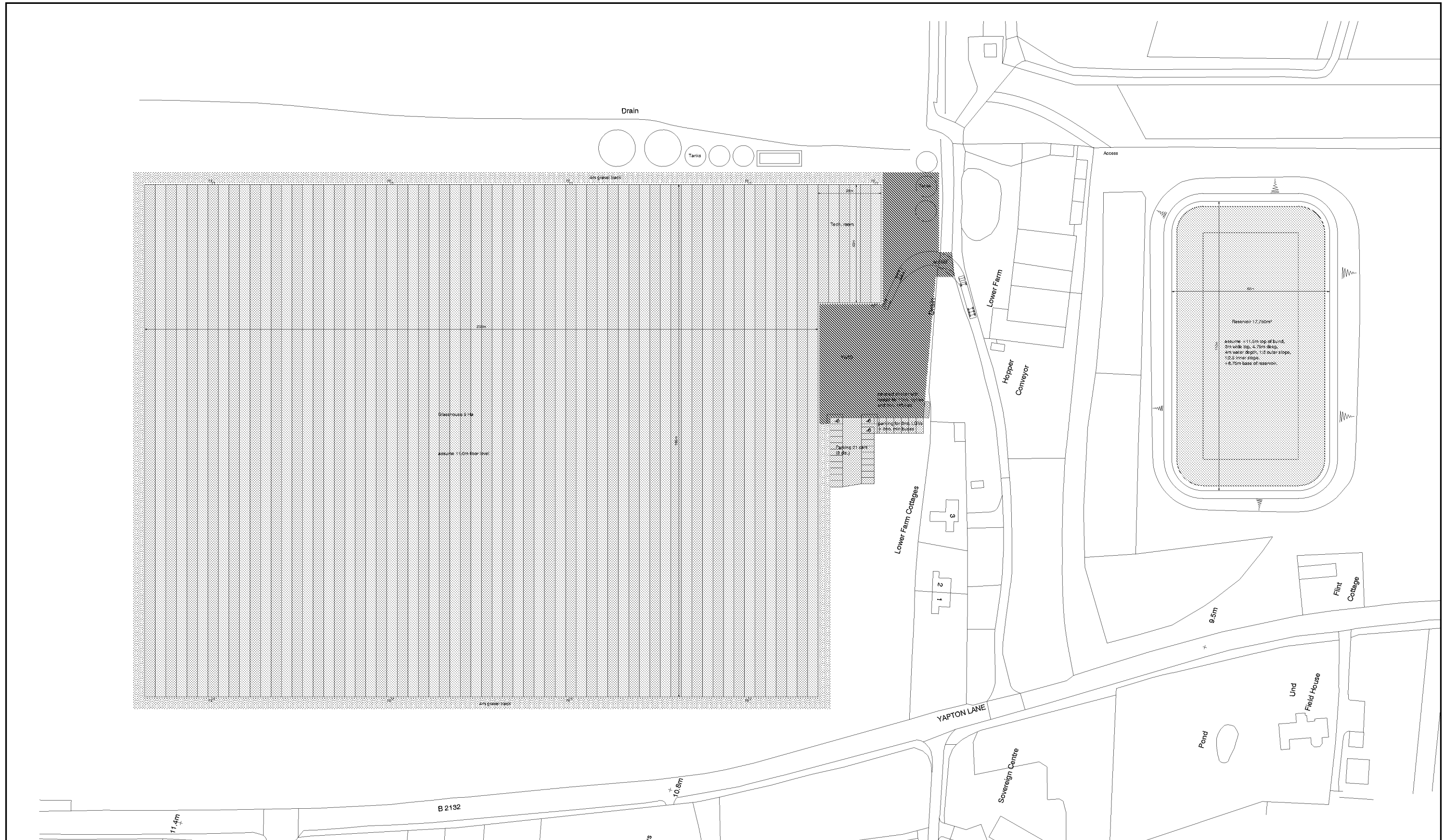
Extract A - Lower Farm Site Block Plan, (Curtis Leeves Technical Drawing No. 2015-PA22 rev P01)
