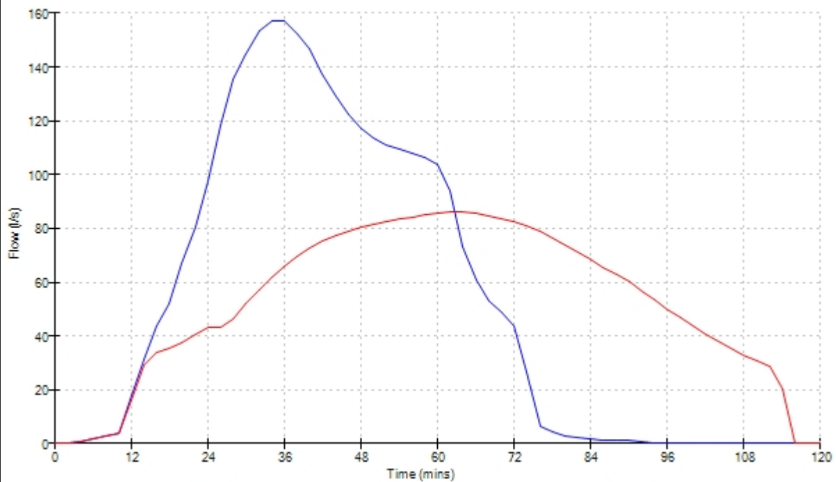
Graphs for Pipe S1.011 US/MH S12 Outlet (15104 GTR FONTWELL.SWS) 60 minute 100 year Winter I+40% Status: SURCHARGED
