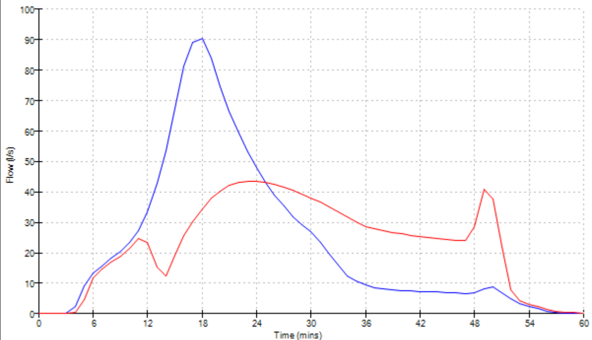
Graphs for Pipe S1.001 US/MH S2 (15104 GTR FONTWELL.SWS) 30 minute 100 year Summer I+40% Status: SURCHARGED
