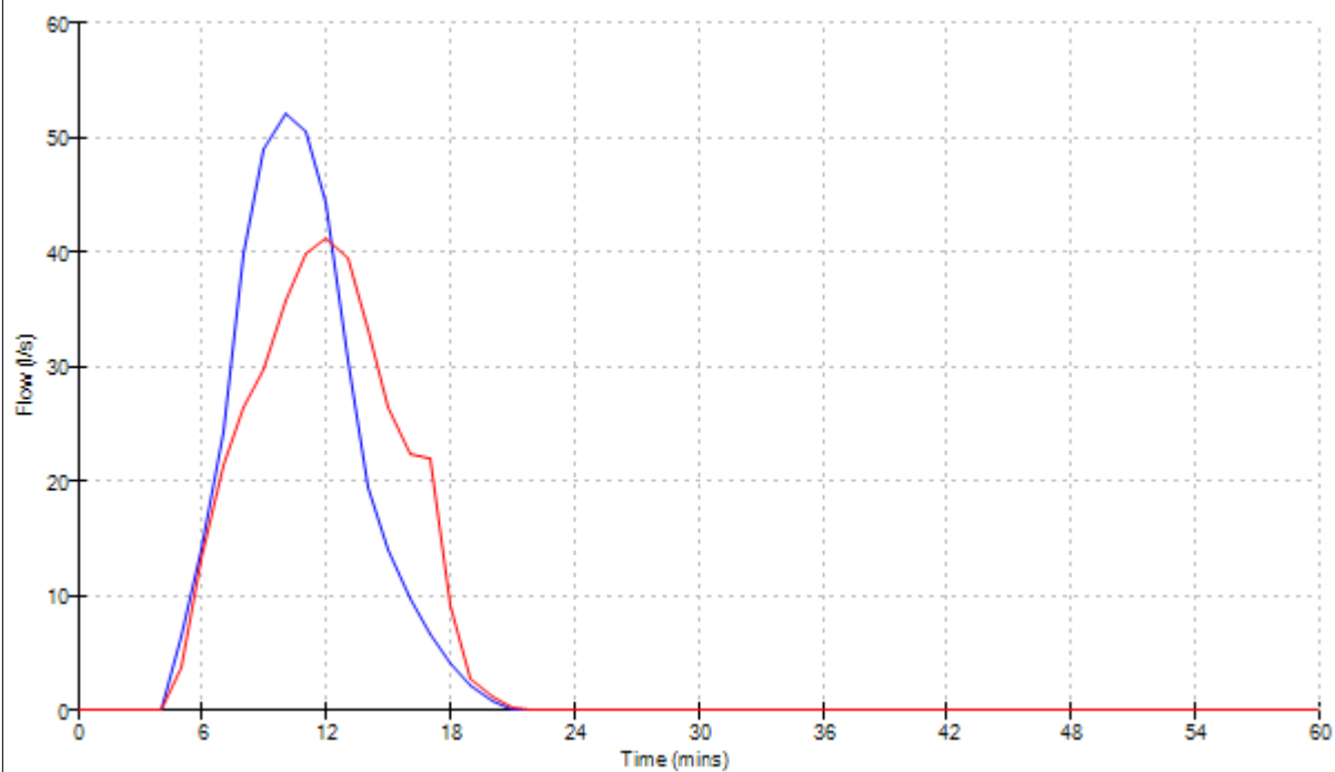
Graphs for Pipe S3.001 US/MH S19 (15104 GTR FONTWELL.SWS) 15 minute 100 year Summer I+40% Status: SURCHARGED
