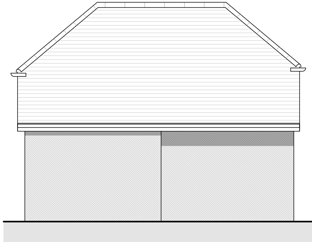
South Elevation
