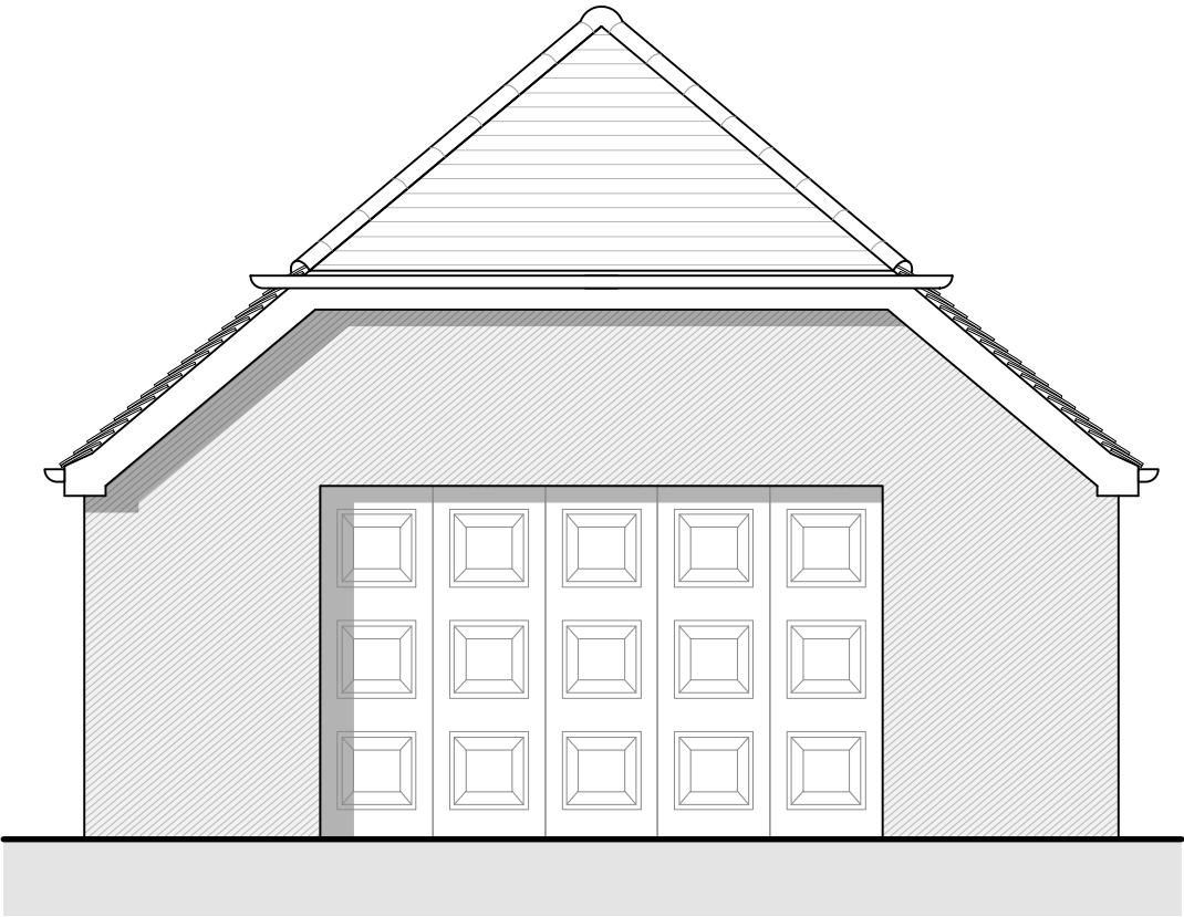
West Elevation
