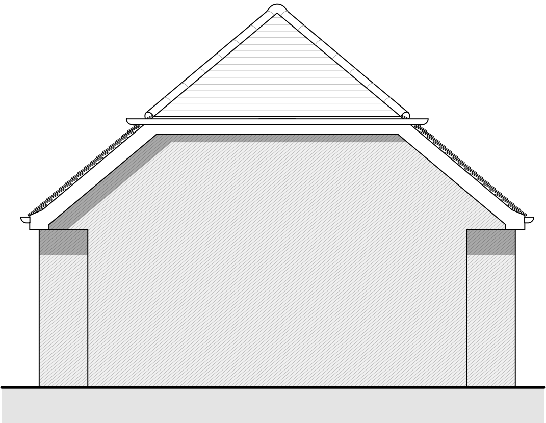
East Elevation
