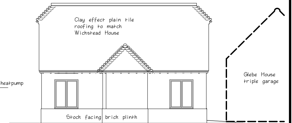
SOUTH EAST ELEVATION 1:100
