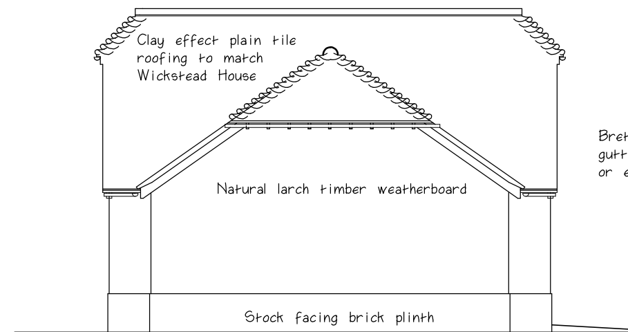
NORTH WEST ELEVATION 1:100
