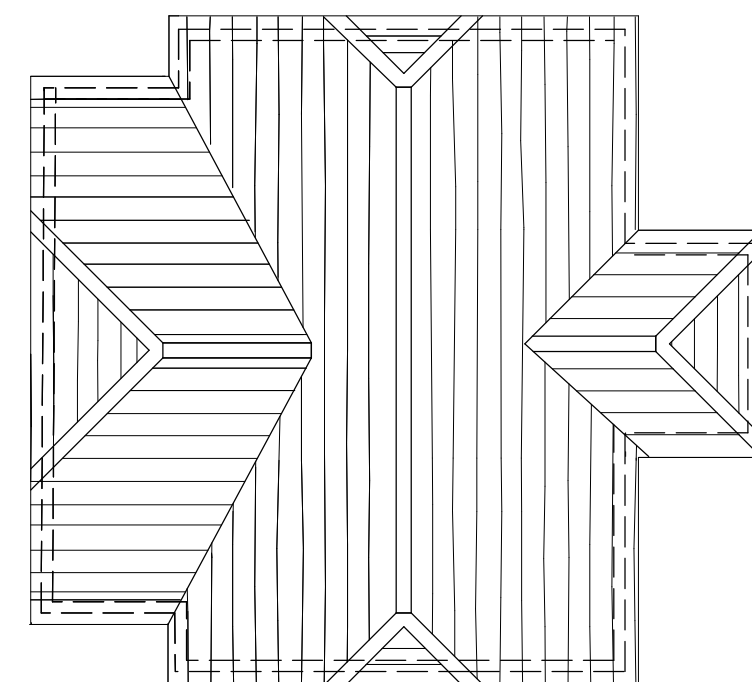
ROOF PLAN 1:100
