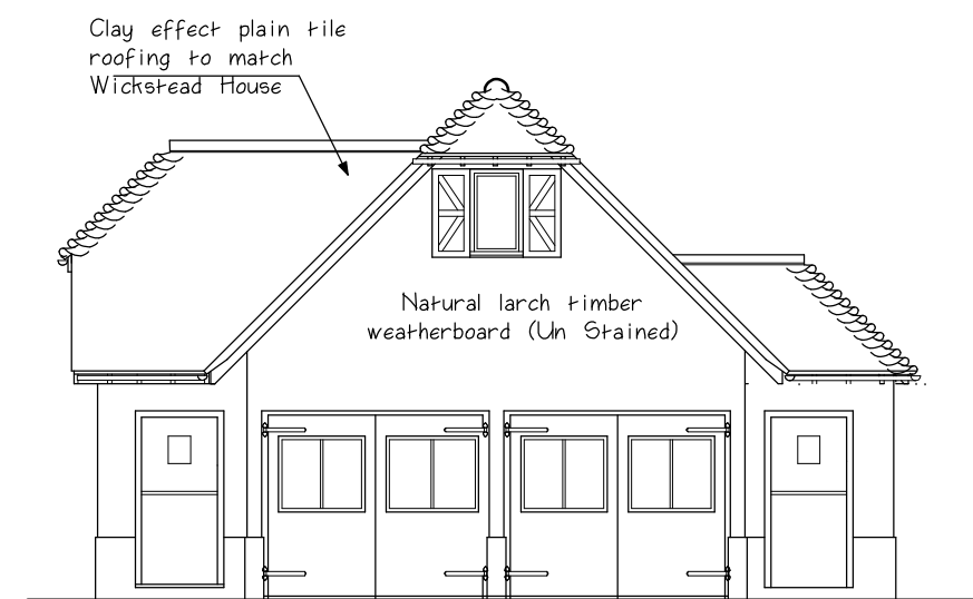
SOUTH WEST ELEVATION 1:100
