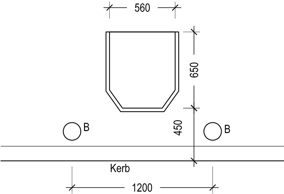
CHARGING POINT PLAN
