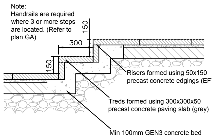
TYPICAL STEPS CONSTRUCTION (Scale 1:20)
