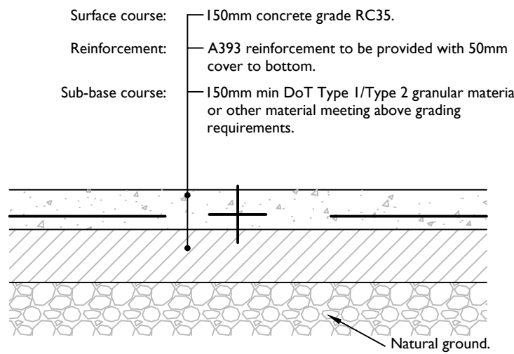
SHED BASE/BIN STORE BASE (Scale 1:20)
