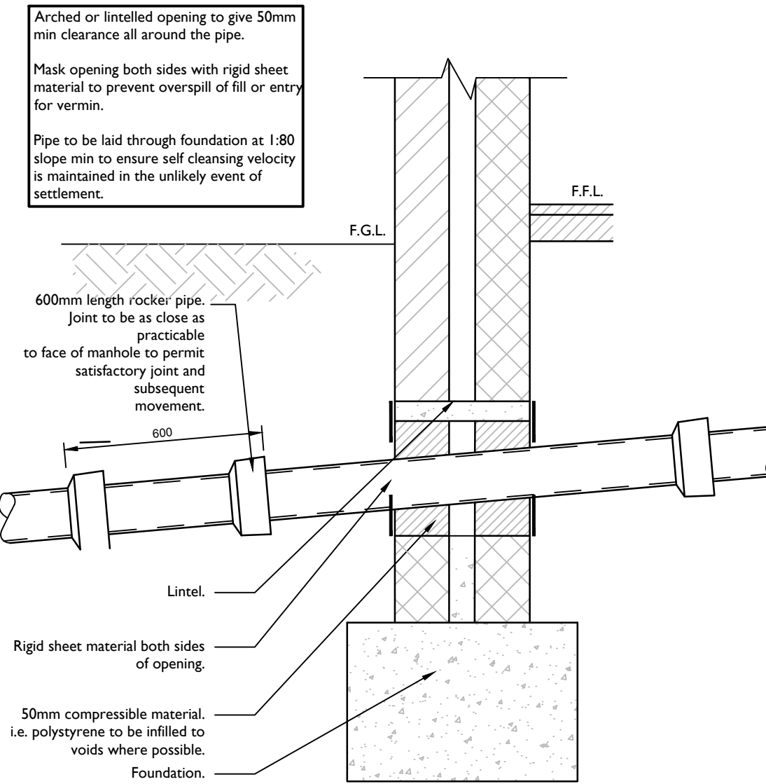
TYPICAL SECTION DETAILING PIPE 'SLEEVE' THROUGH LINTEL OPENING (Scale 1:20)
