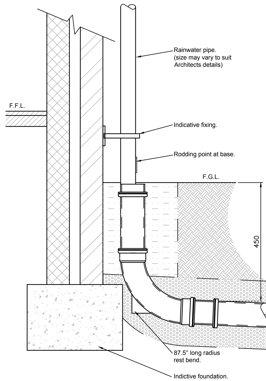
DETAIL OF RAINWATER PIPE (Scale 1:20)
