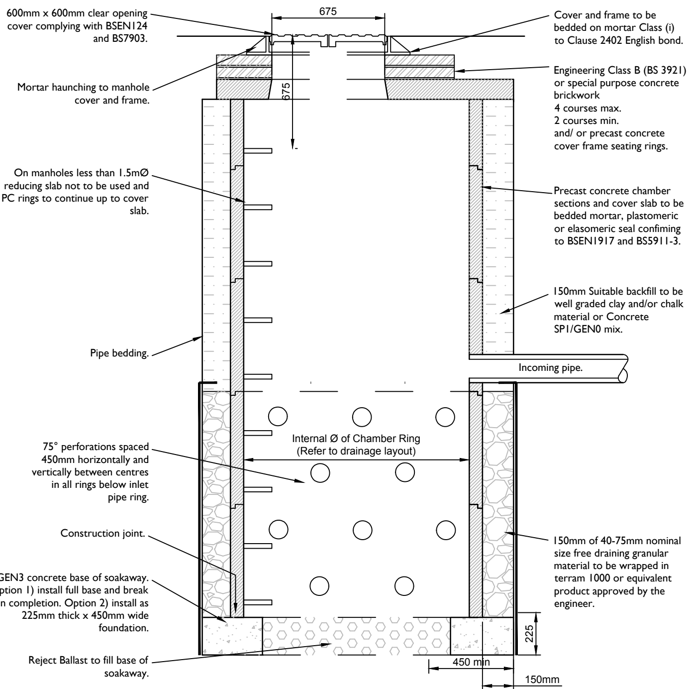
DETAIL OF PRECAST CONCRETE PERFORATED RING SOAKAWAY (DEPTHS LESS THAN 3.0m) (Scale 1:20)
