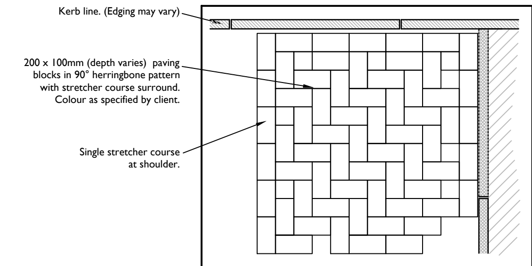
BLOCK PAVING ARRANGEMENT PLAN (Scale 1:20)
