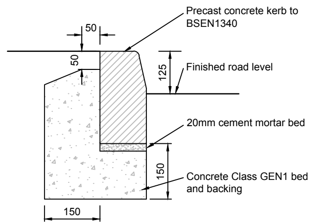
HB2 KERB (1:10)
