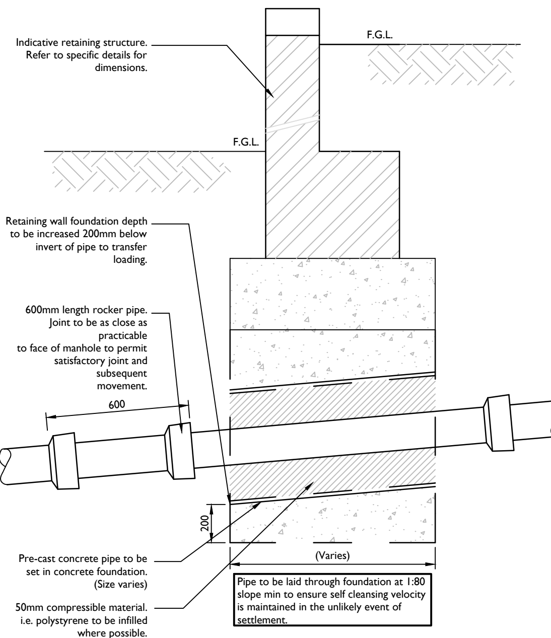
TYPICAL SECTION DETAILING PIPE 'SLEEVE' THROUGH BRICKWORK RETAINING WALL/FOUNDATION (Scale 1:20)
