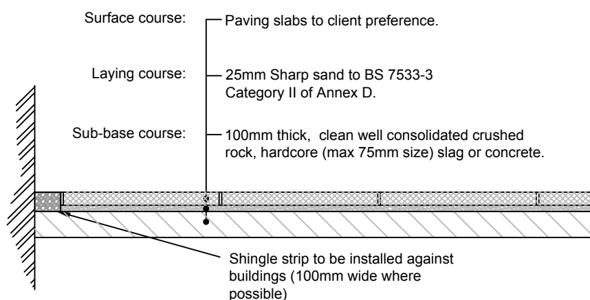
PRIVATE PATIO/FOOTPATH CONSTRUCTION (Scale 1:20)
