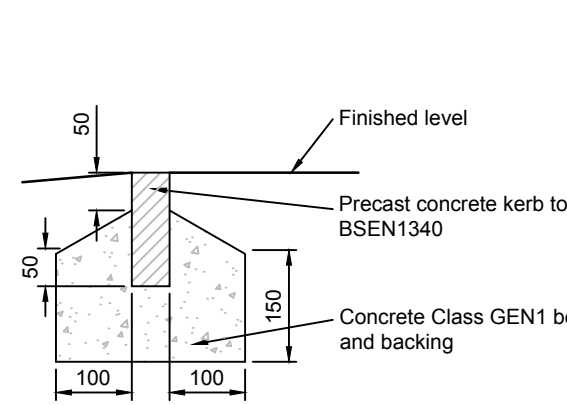
EF EDGING (1:10)
