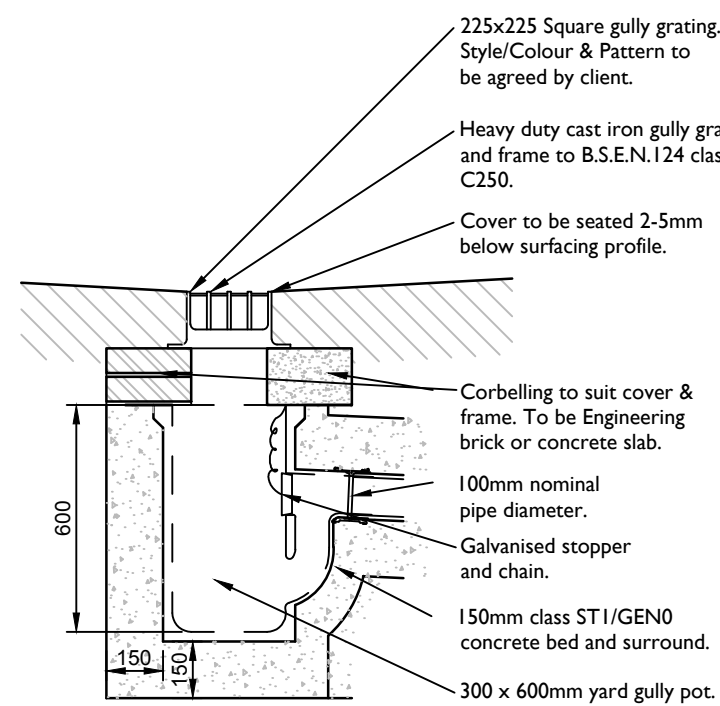
TYPICAL YARD GULLY (600mm POT) (Scale 1:20)
