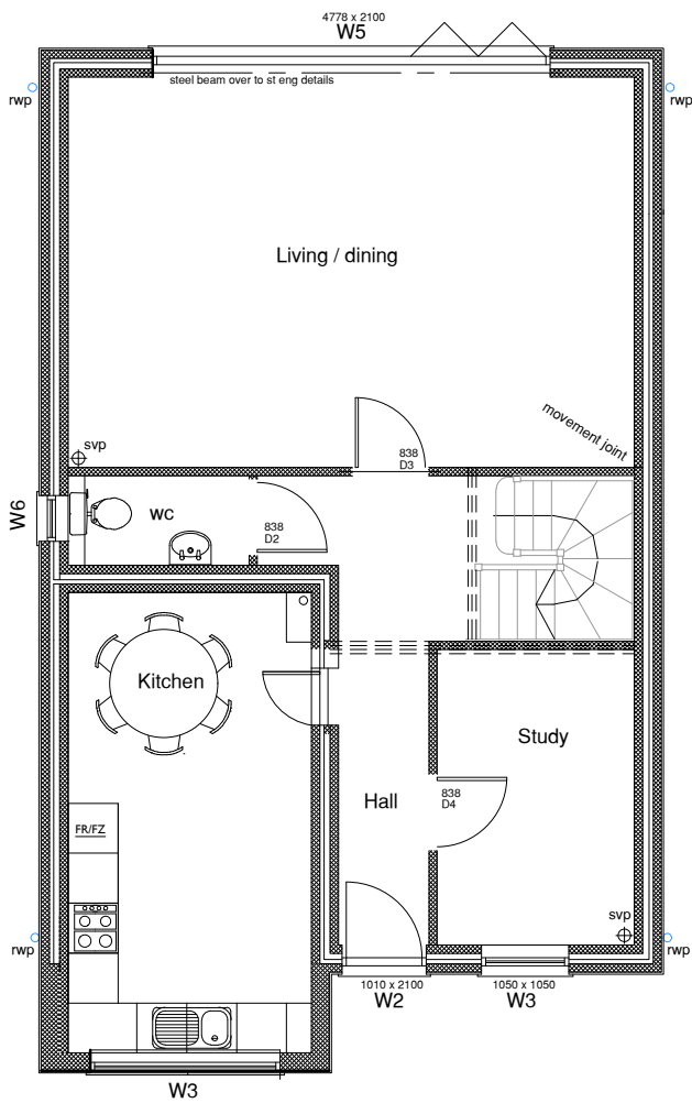
PROPOSED GROUND FLOOR PLAN Plots 5 & 6
