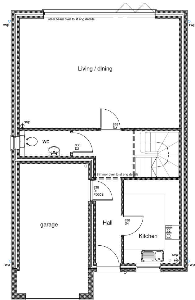
EXISTING GROUND FLOOR PLAN Plots 5 & 6
