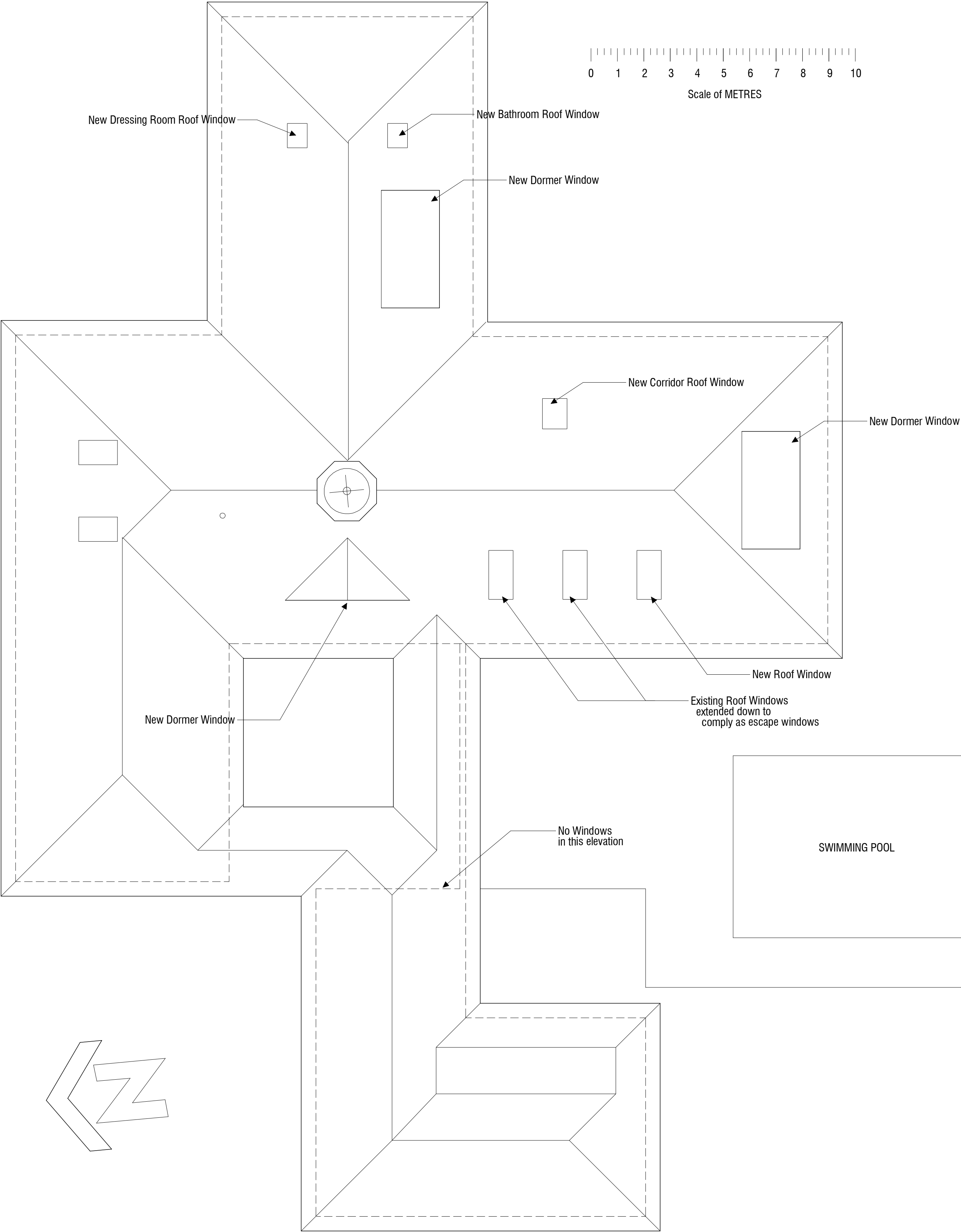
ROOF PLAN as Proposed
