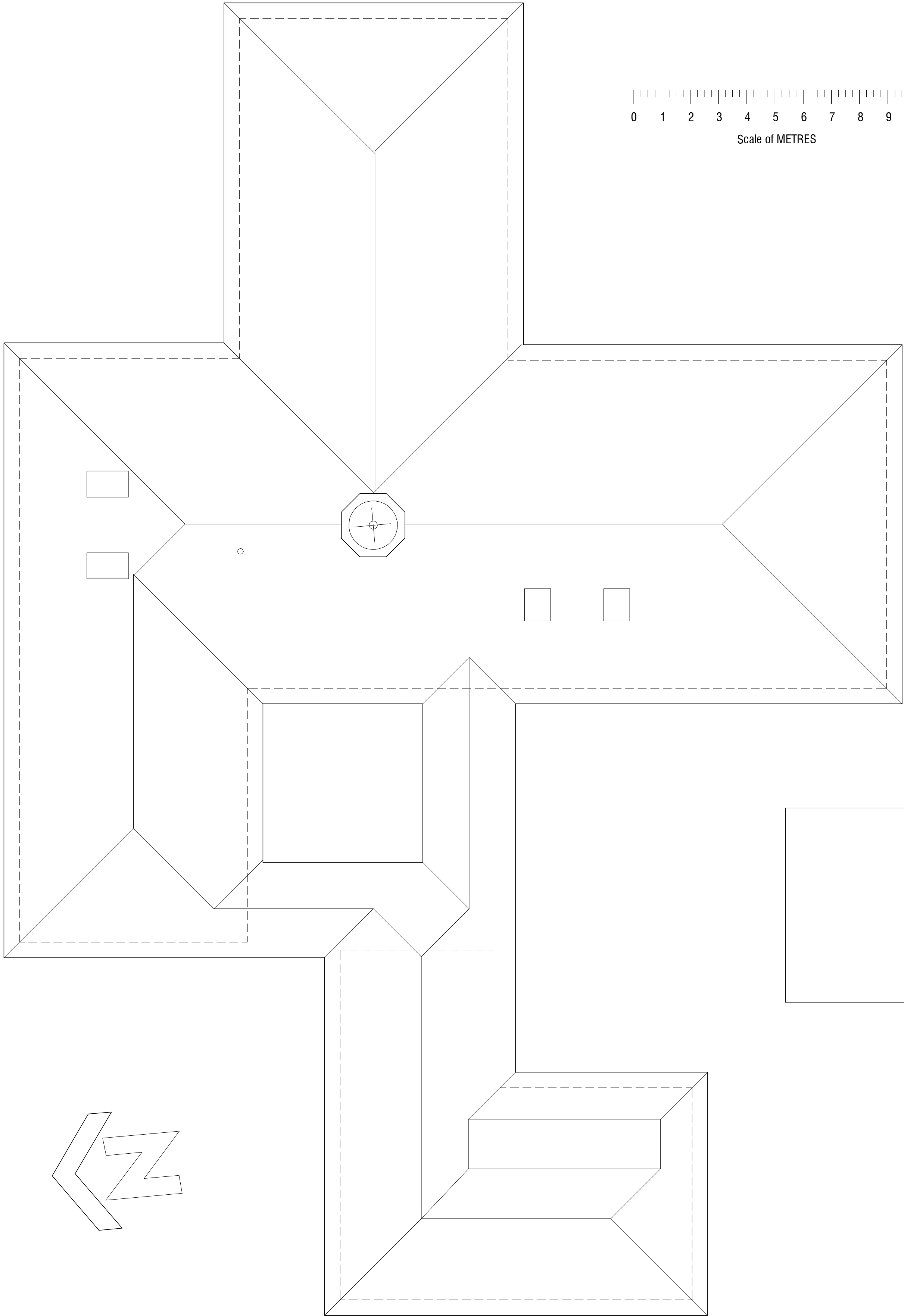
ROOF PLAN as Existing
