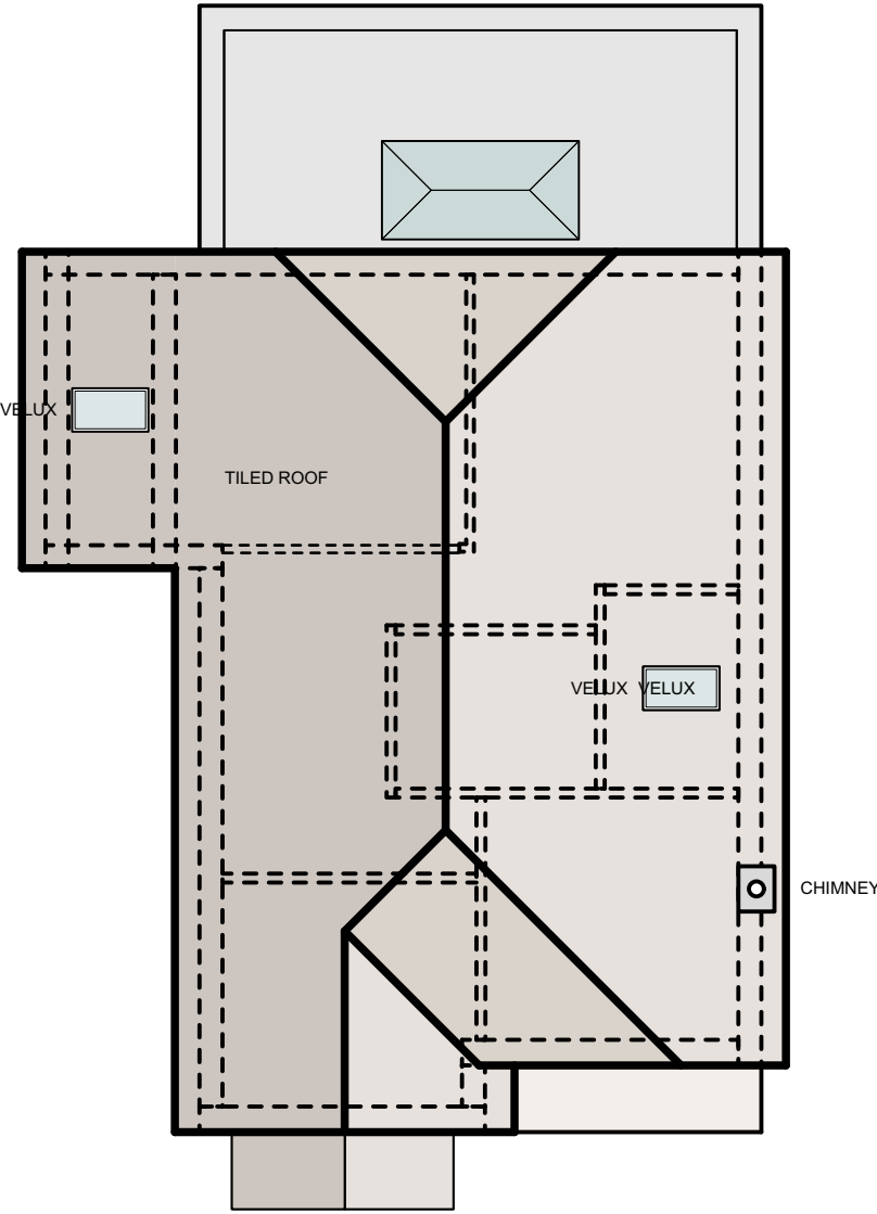
roof plan:
