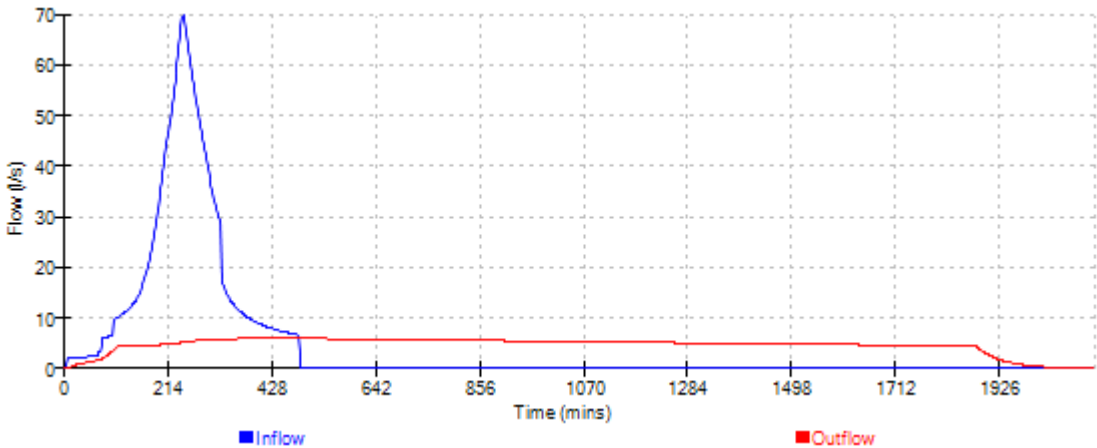
Cascade Event: 480 min Summer for 15104 Soakaway cascade Rev B.SRCX
