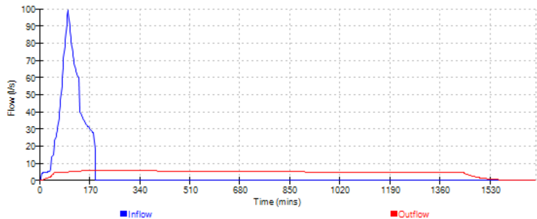
Cascade Event: 180 min Summer for 15104 Soakaway cascade Rev B.SRCX
