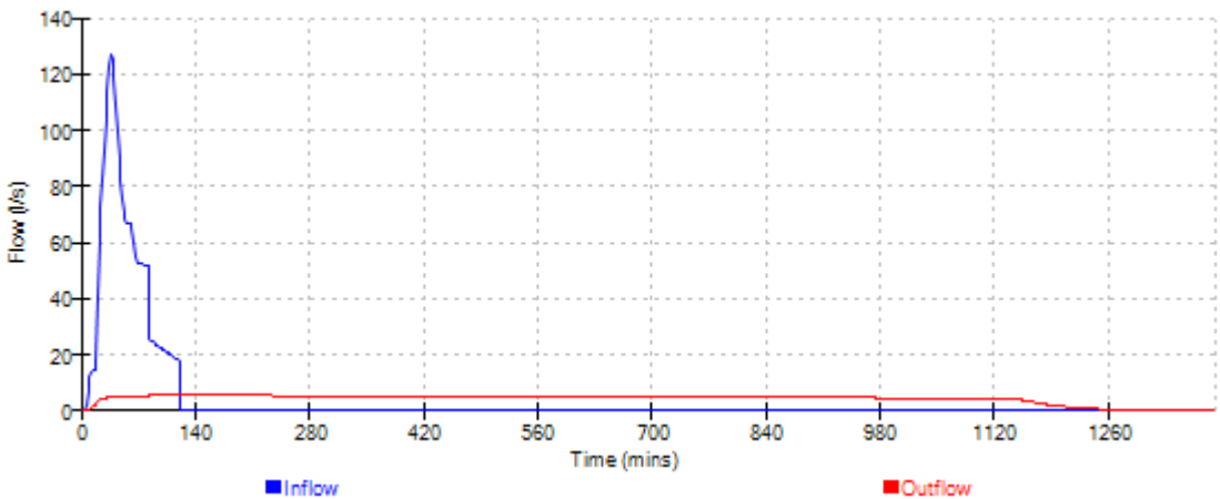
Cascade Event: 60 min Winter for 15104 Soakaway cascade Rev B.SRCX
