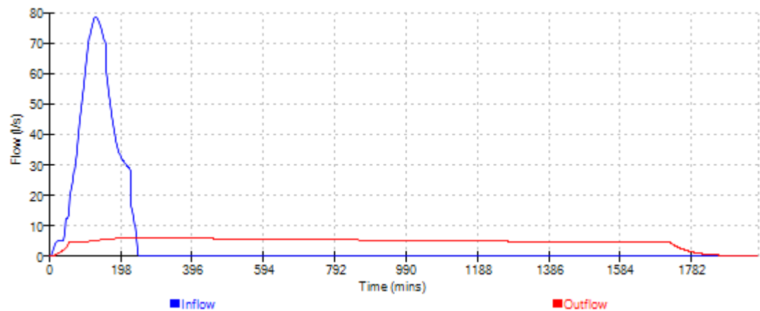
Cascade Event: 240 min Winter for 15104 Soakaway cascade Rev B.SRCX
