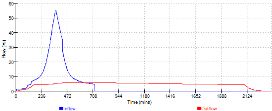
Cascade Event: 720 min Summer for 15104 Soakaway cascade Rev B.SRCX
