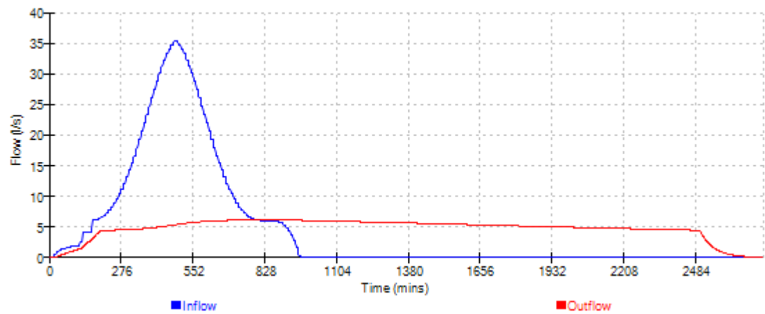
Cascade Event: 960 min Winter for 15104 Soakaway cascade Rev B.SRCX
