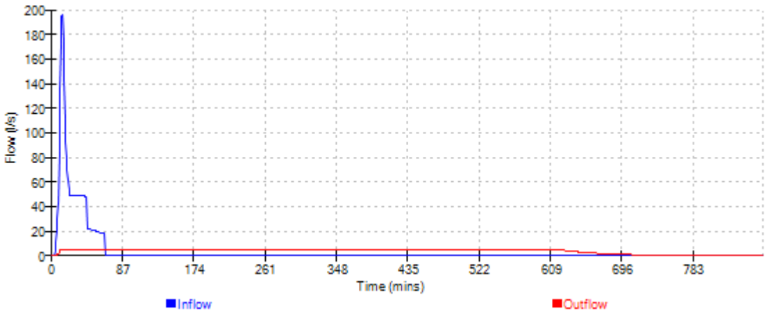
Cascade Event: 15 min Winter for 15104 Soakaway cascade Rev B.SRCX
